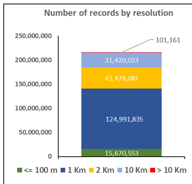
Fig. 1. Number of records by resolution
